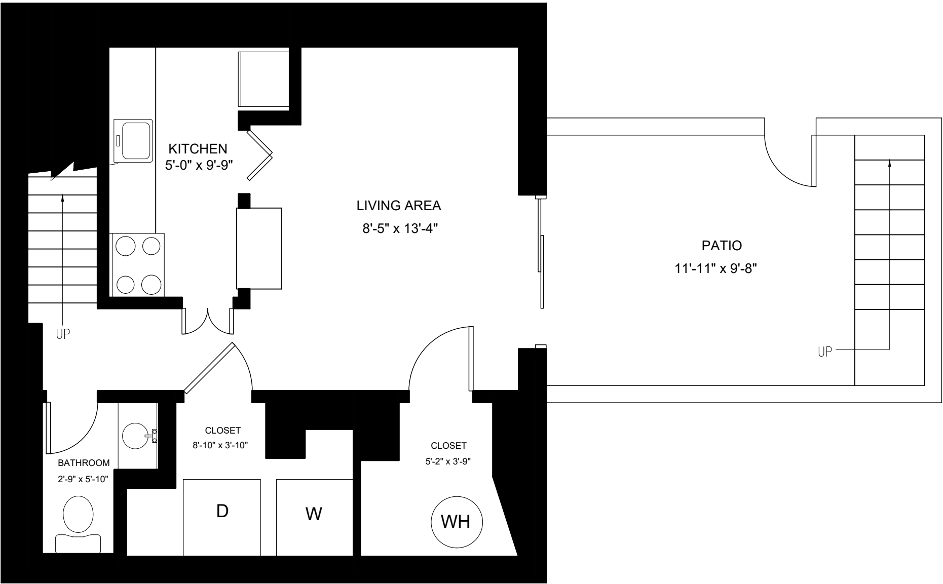
BASEMENT
