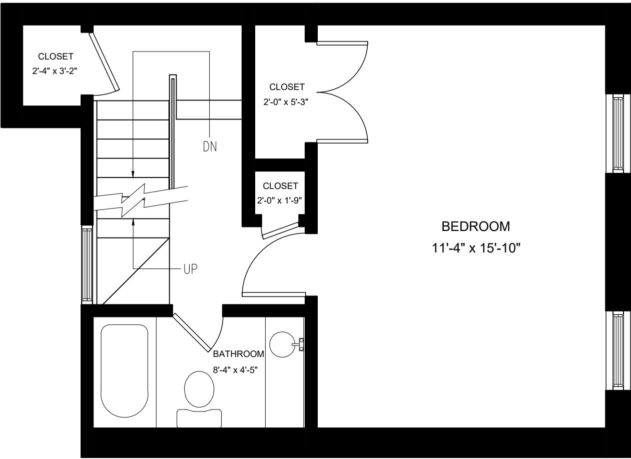
SECOND FLOOR
